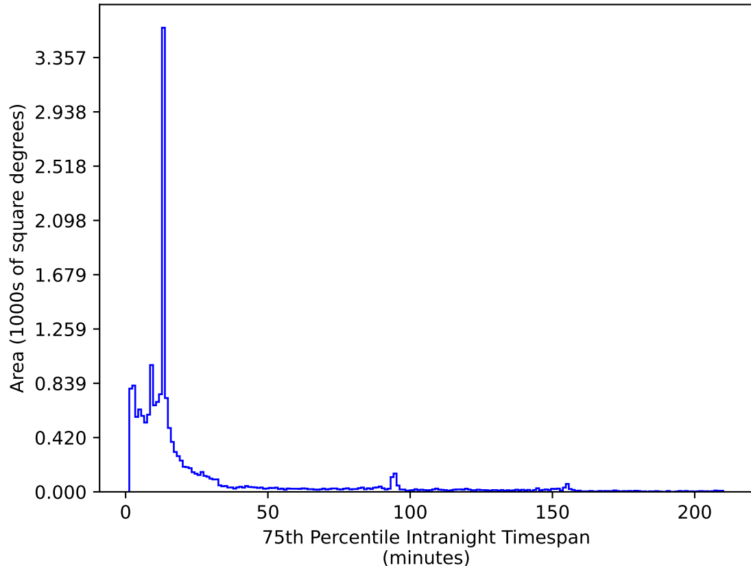
too_elab_r8_d2_giz_v3.4_10yrs WFD z band: 75th Percentile Intranight Timespan
