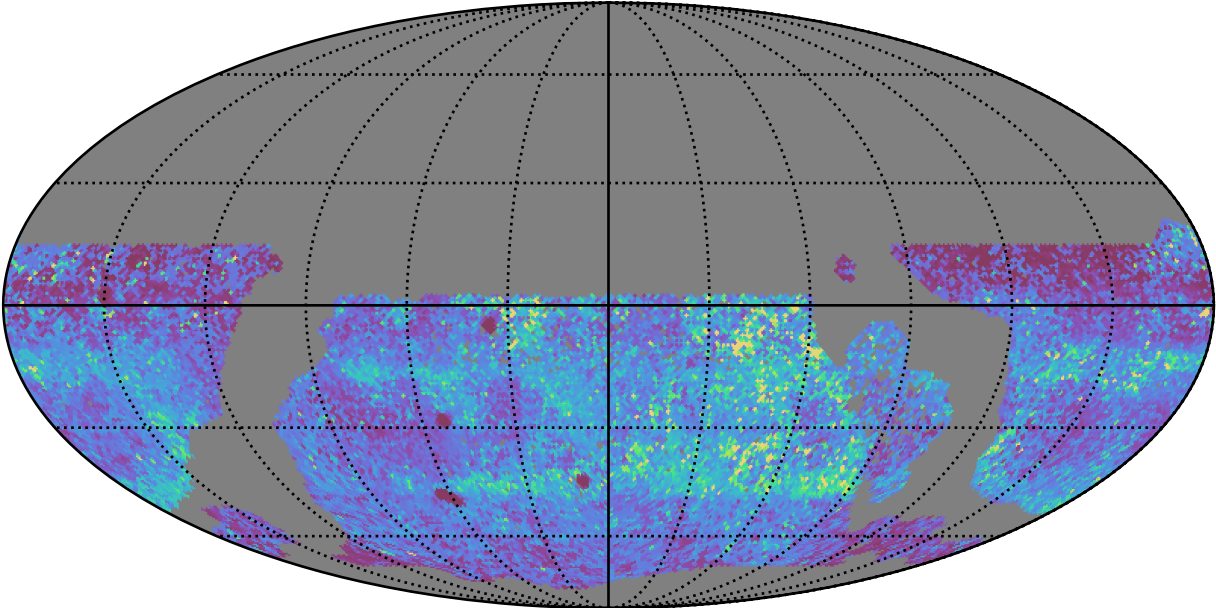
too_elab_r8_d2_giz_v3.4_10yrs WFD y band: 75th Percentile Intranight Timespan
