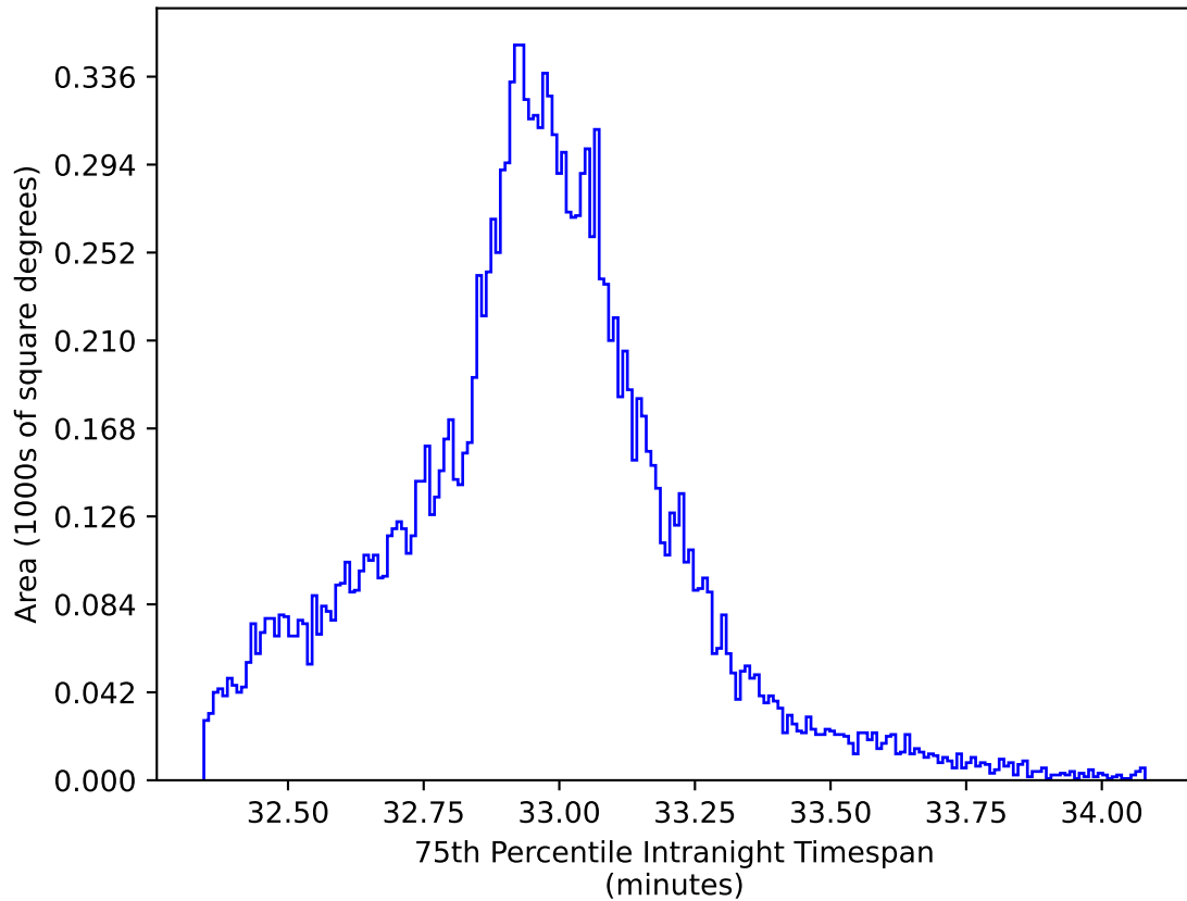
too_elab_r8_d2_giz_v3.4_10yrs WFD y band: 75th Percentile Intranight Timespan
