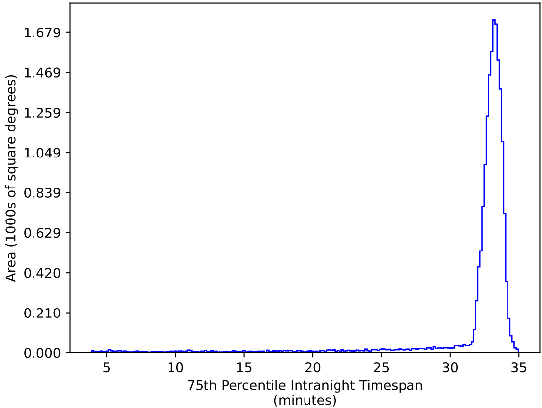
too_elab_r8_d2_giz_v3.4_10yrs WFD ug bands: 75th Percentile Intranight Timespan
