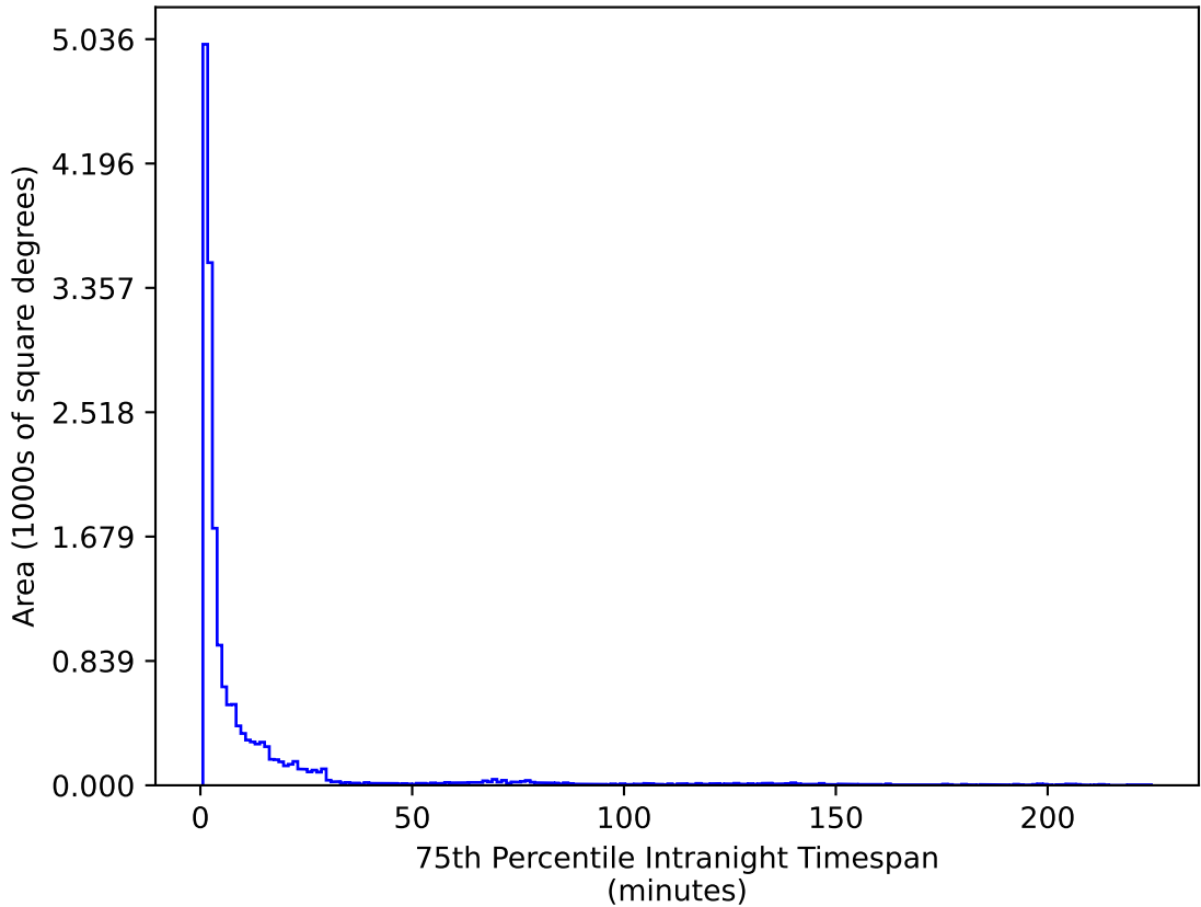
too_elab_r8_d2_giz_v3.4_10yrs WFD u band: 75th Percentile Intranight Timespan
