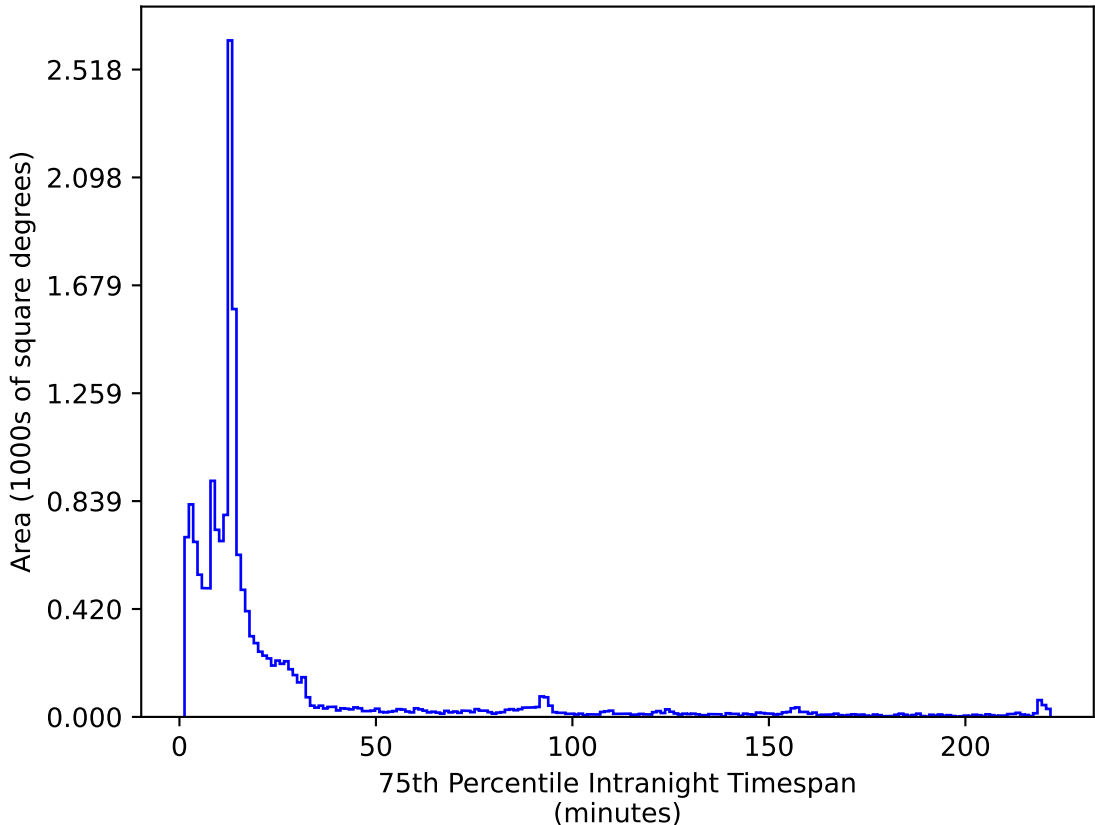
too_elab_r8_d2_giz_v3.4_10yrs WFD i band: 75th Percentile Intranight Timespan
