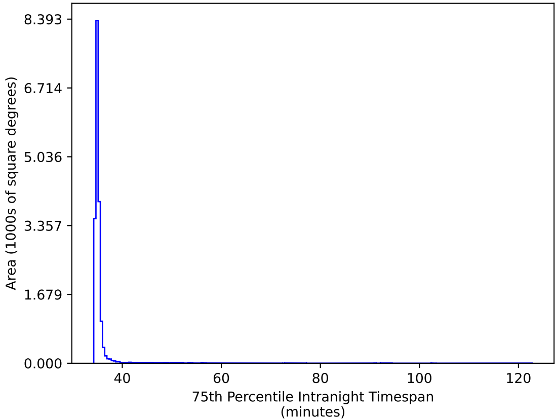
too_elab_r8_d2_giz_v3.4_10yrs WFD gr bands: 75th Percentile Intranight Timespan
