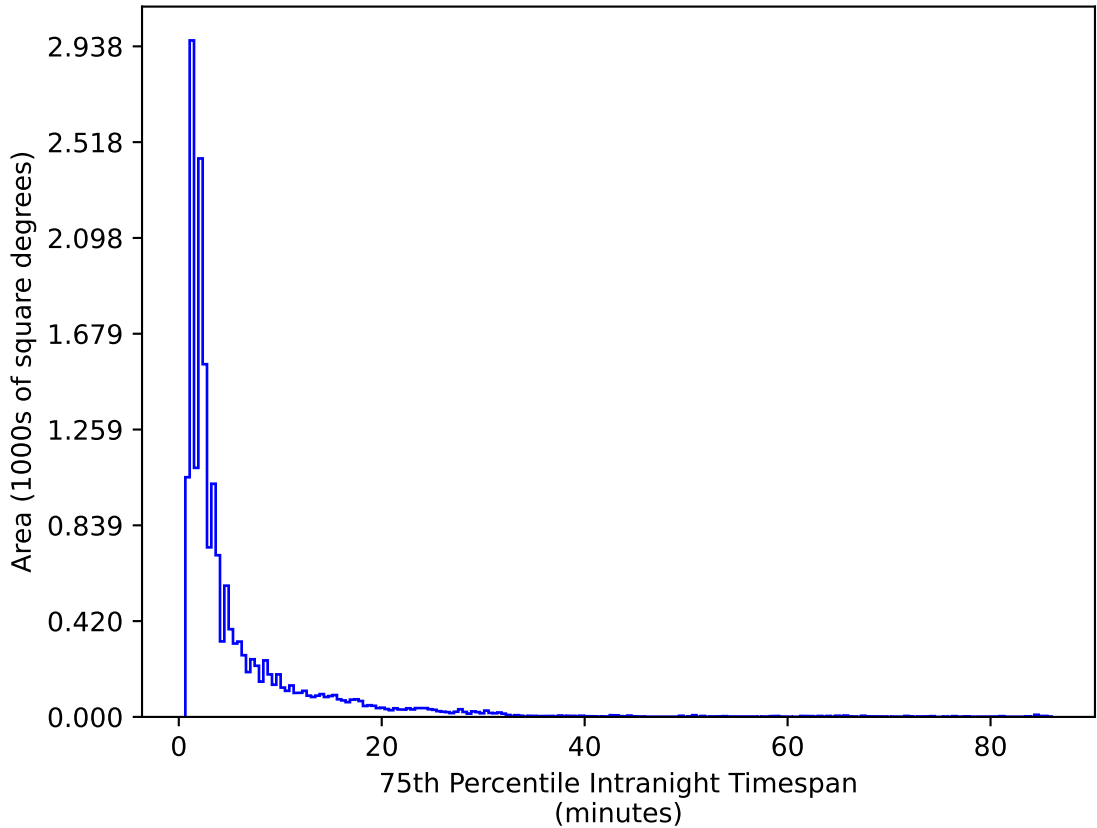
too_elab_r8_d2_giz_v3.4_10yrs WFD g band: 75th Percentile Intranight Timespan
