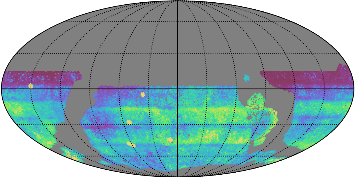
too_elab_r8_d2_giz_v3.4_10yrs WFD all bands: 75th Percentile Intranight Timespan
