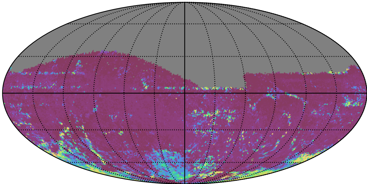
too_elab_r8_d2_giz_v3.4_10yrs All sky z band: 75th Percentile Intranight Timespan
