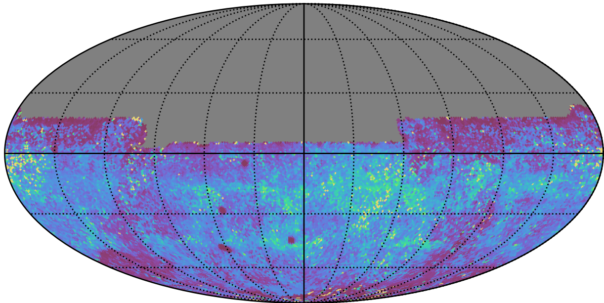
too_elab_r8_d2_giz_v3.4_10yrs All sky y band: 75th Percentile Intranight Timespan
