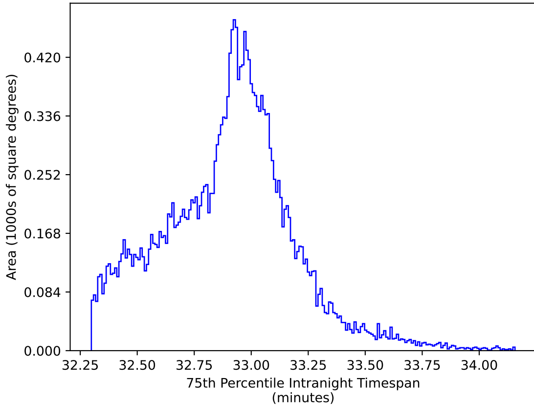
too_elab_r8_d2_giz_v3.4_10yrs All sky y band: 75th Percentile Intranight Timespan
