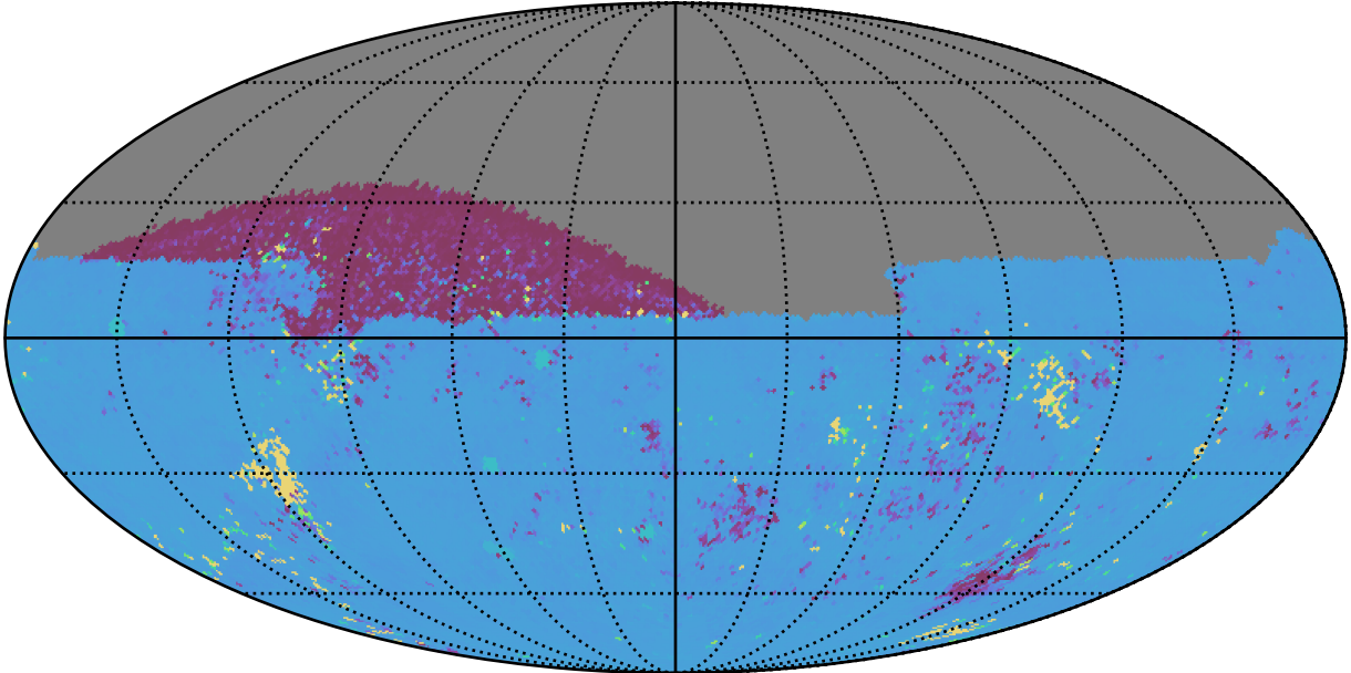
too_elab_r8_d2_giz_v3.4_10yrs All sky ug bands: 75th Percentile Intranight Timespan
