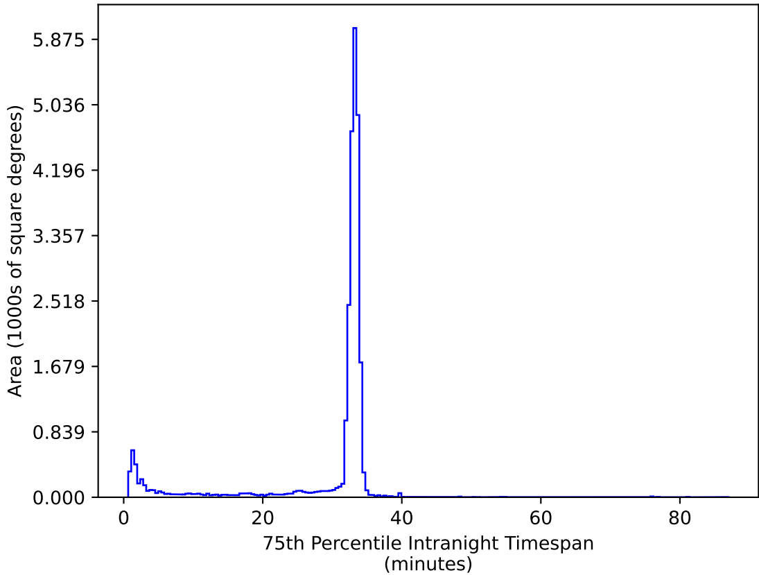
too_elab_r8_d2_giz_v3.4_10yrs All sky ug bands: 75th Percentile Intranight Timespan
