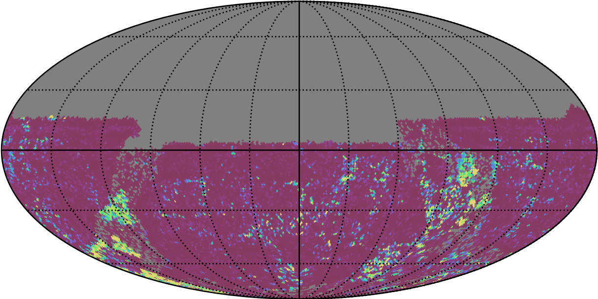
too_elab_r8_d2_giz_v3.4_10yrs All sky u band: 75th Percentile Intranight Timespan
