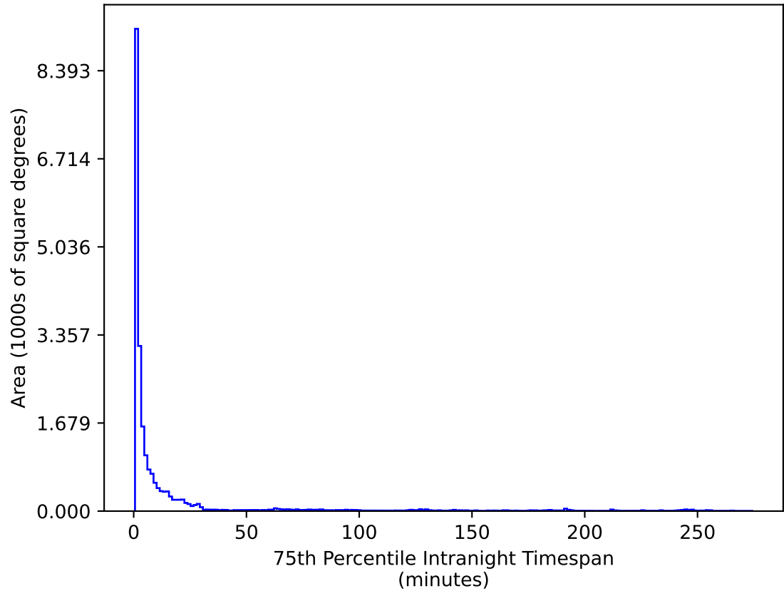
too_elab_r8_d2_giz_v3.4_10yrs All sky u band: 75th Percentile Intranight Timespan
