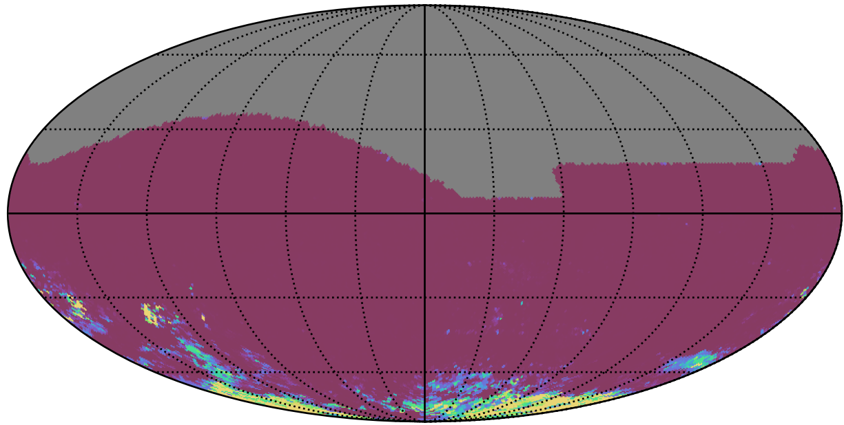
too_elab_r8_d2_giz_v3.4_10yrs All sky ri bands: 75th Percentile Intranight Timespan
