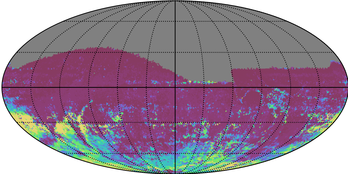
too_elab_r8_d2_giz_v3.4_10yrs All sky r band: 75th Percentile Intranight Timespan
