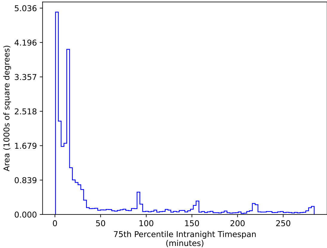
too_elab_r8_d2_giz_v3.4_10yrs All sky r band: 75th Percentile Intranight Timespan
