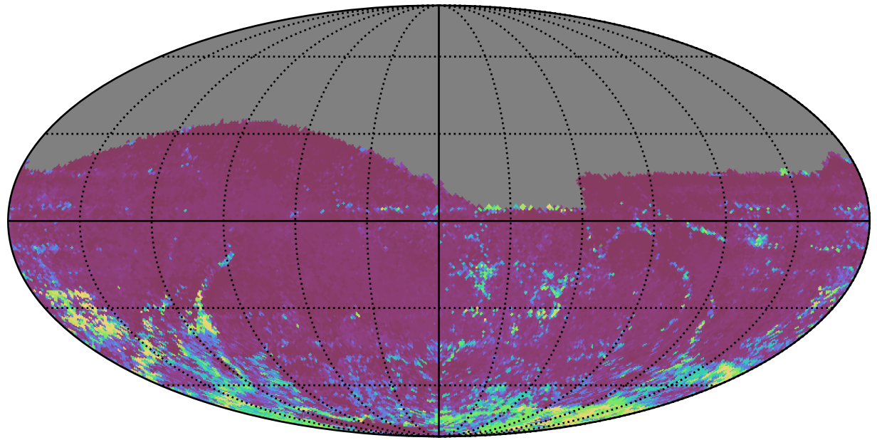
too_elab_r8_d2_giz_v3.4_10yrs All sky i band: 75th Percentile Intranight Timespan
