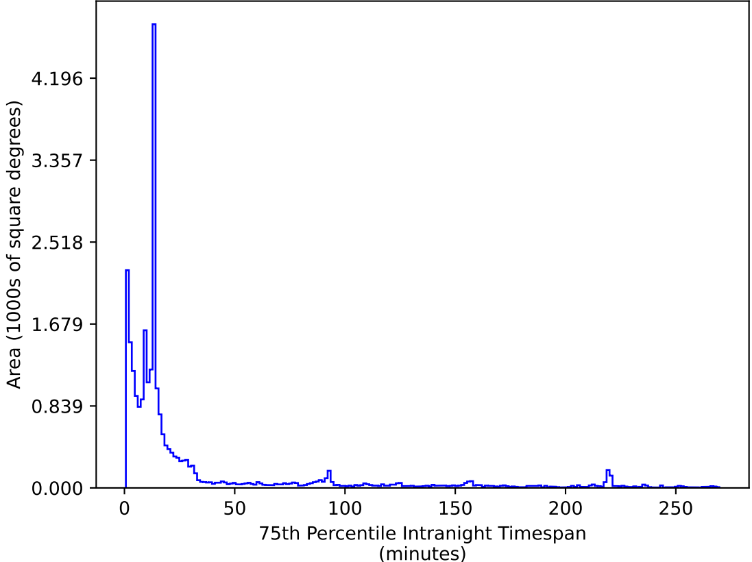
too_elab_r8_d2_giz_v3.4_10yrs All sky i band: 75th Percentile Intranight Timespan
