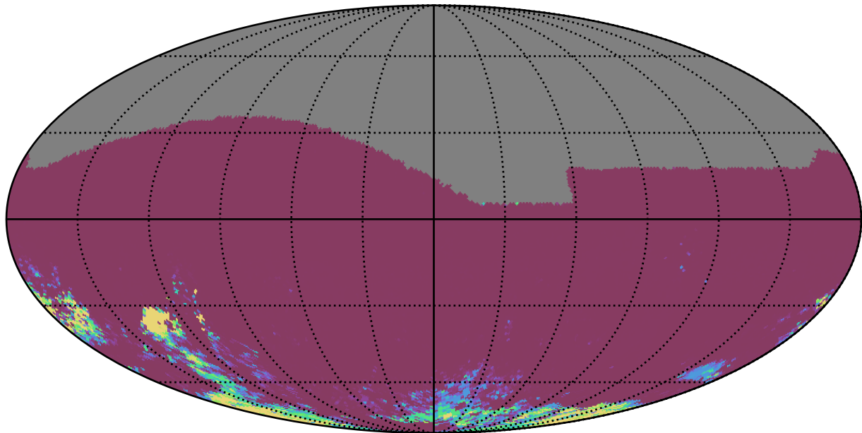
too_elab_r8_d2_giz_v3.4_10yrs All sky gr bands: 75th Percentile Intranight Timespan
