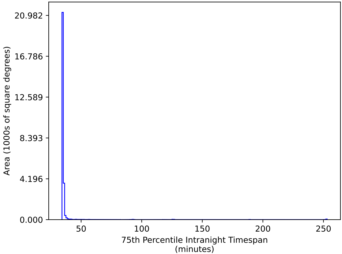
too_elab_r8_d2_giz_v3.4_10yrs All sky gr bands: 75th Percentile Intranight Timespan
