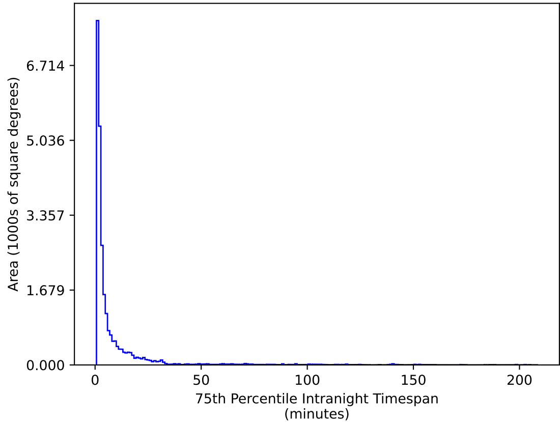
too_elab_r8_d2_giz_v3.4_10yrs All sky g band: 75th Percentile Intranight Timespan
