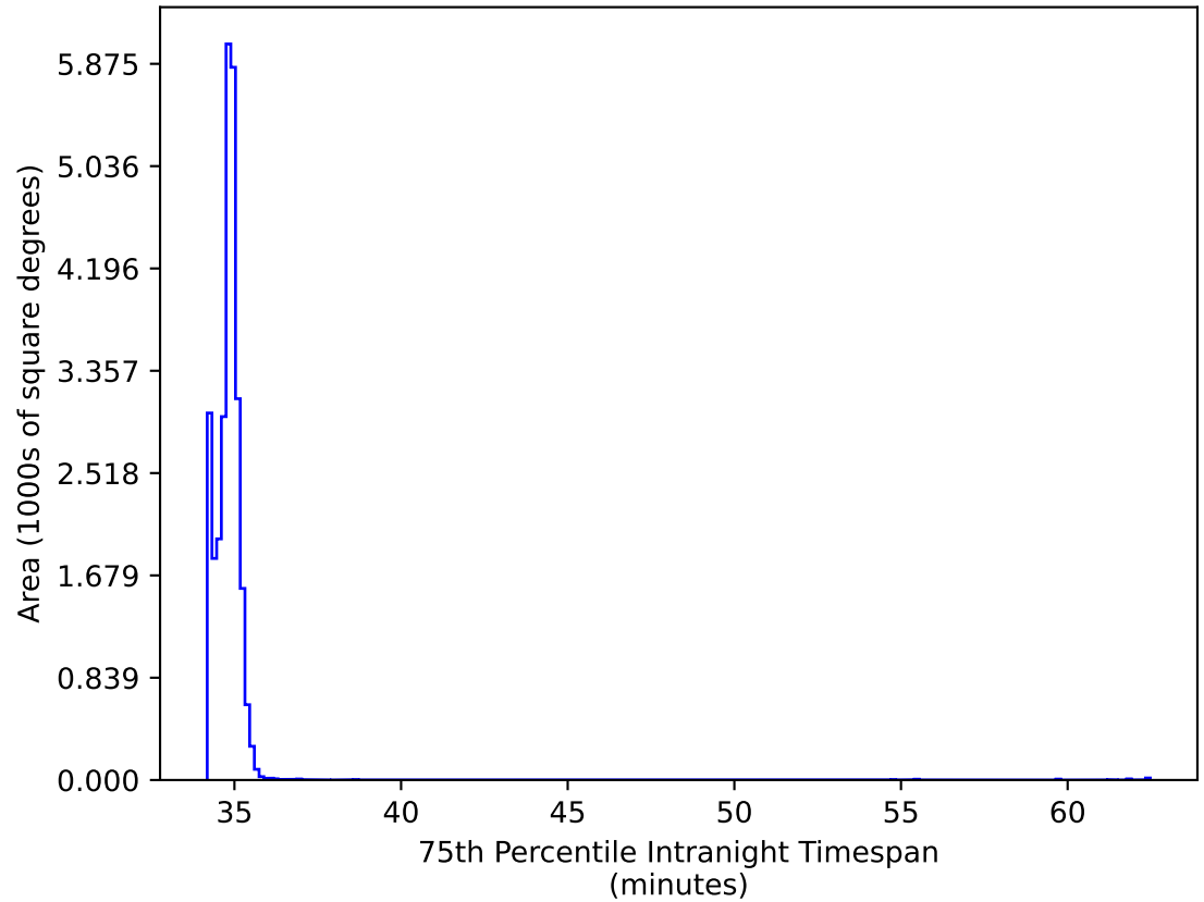
too_elab_r8_d2_giz_v3.4_10yrs All sky all bands: 75th Percentile Intranight Timespan
