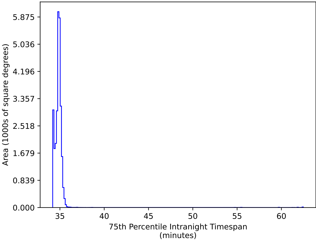
too_elab_r8_d2_giz_v3.4_10yrs All sky: 75th Percentile Intranight Timespan
