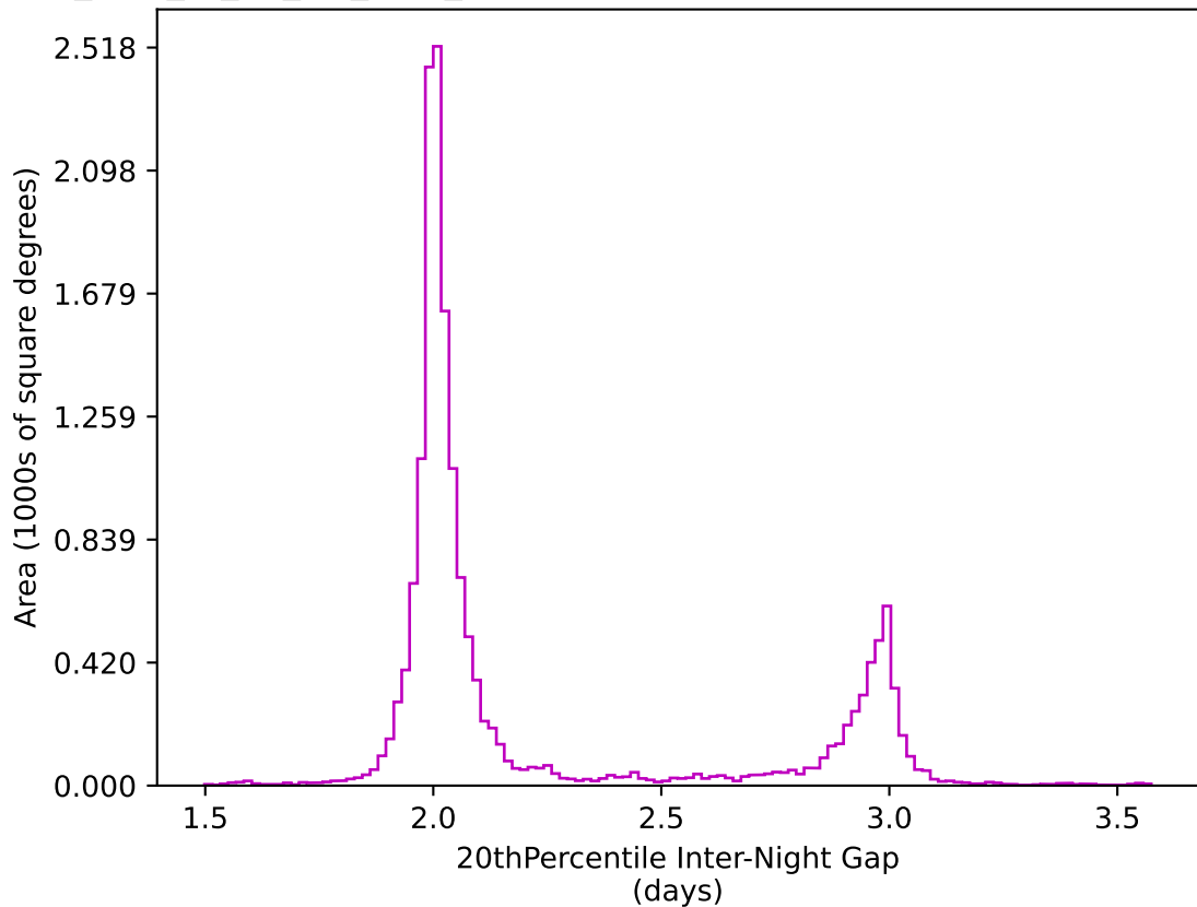
too_elab_r8_d2_giz_v3.4_10yrs WFD z band: 20thPercentile Inter-Night Gap
