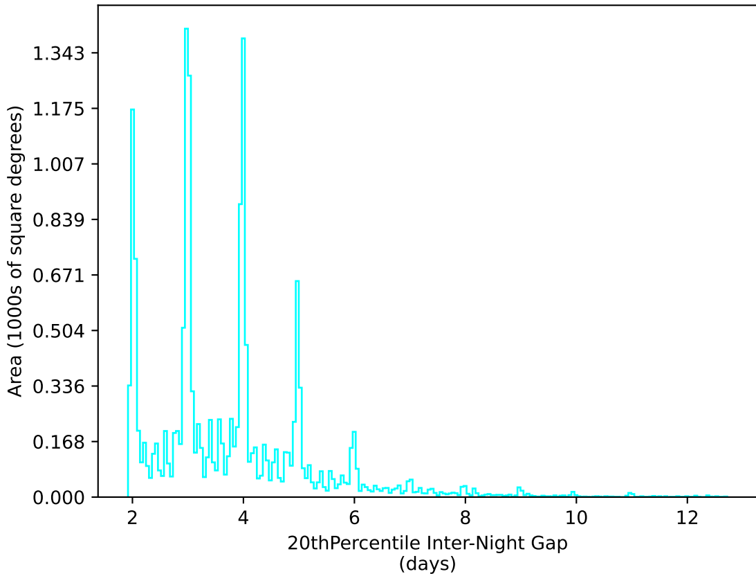
too_elab_r8_d2_giz_v3.4_10yrs WFD u band: 20thPercentile Inter-Night Gap
