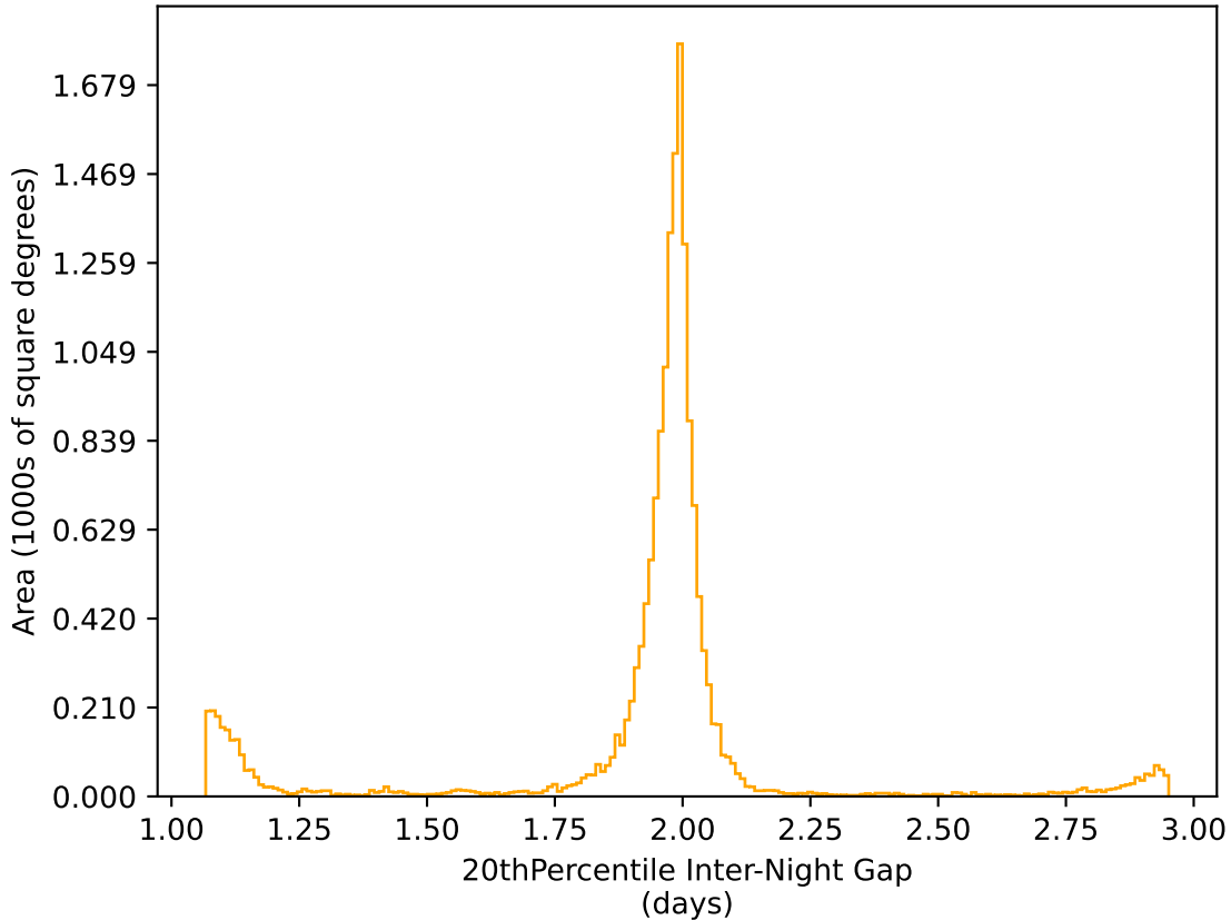
too_elab_r8_d2_giz_v3.4_10yrs WFD r band: 20thPercentile Inter-Night Gap
