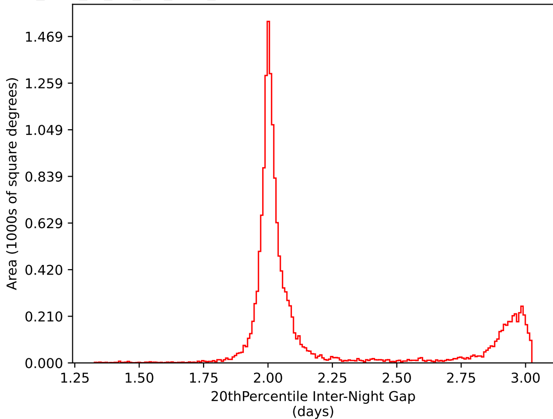
too_elab_r8_d2_giz_v3.4_10yrs WFD i band: 20thPercentile Inter-Night Gap
