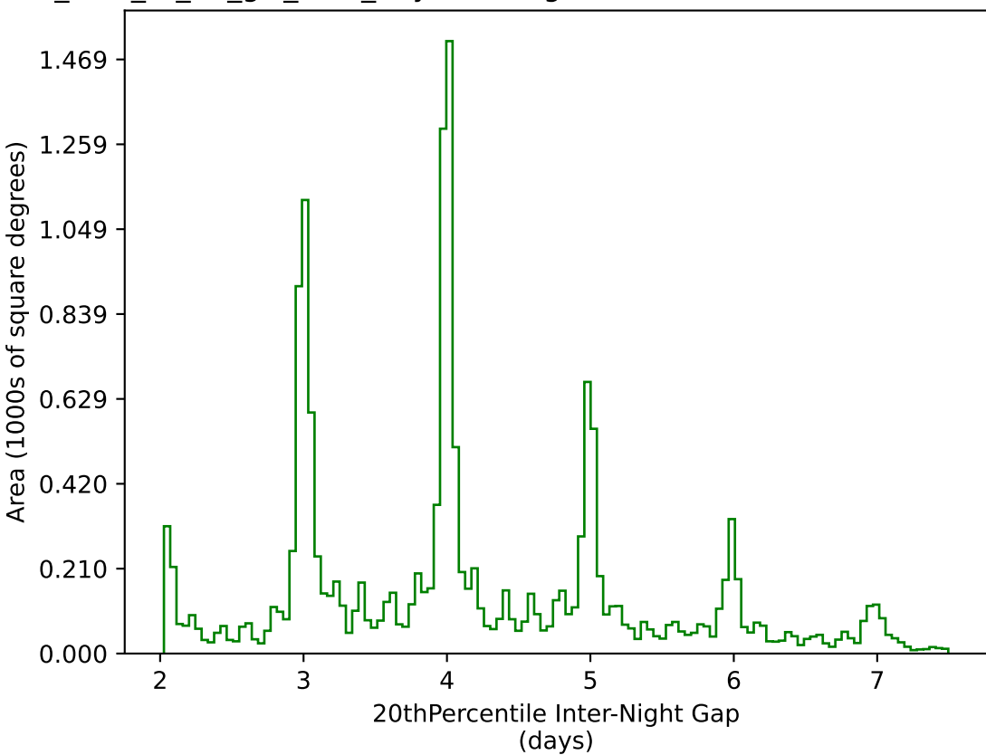
too_elab_r8_d2_giz_v3.4_10yrs WFD g band: 20thPercentile Inter-Night Gap
