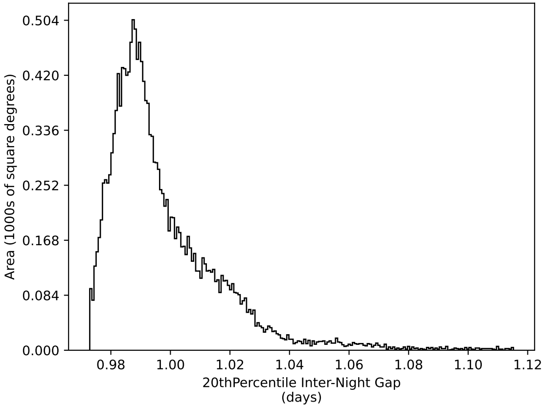
too_elab_r8_d2_giz_v3.4_10yrs WFD all bands: 20thPercentile Inter-Night Gap
