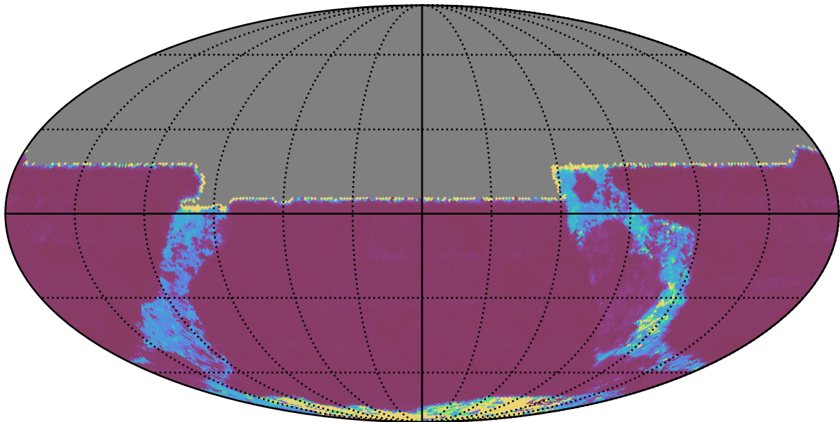
too_elab_r8_d2_giz_v3.4_10yrs All sky y band: 20thPercentile Inter-Night Gap
