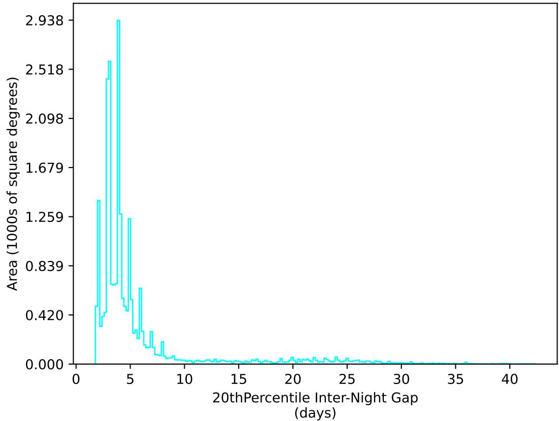
too_elab_r8_d2_giz_v3.4_10yrs All sky u band: 20thPercentile Inter-Night Gap
