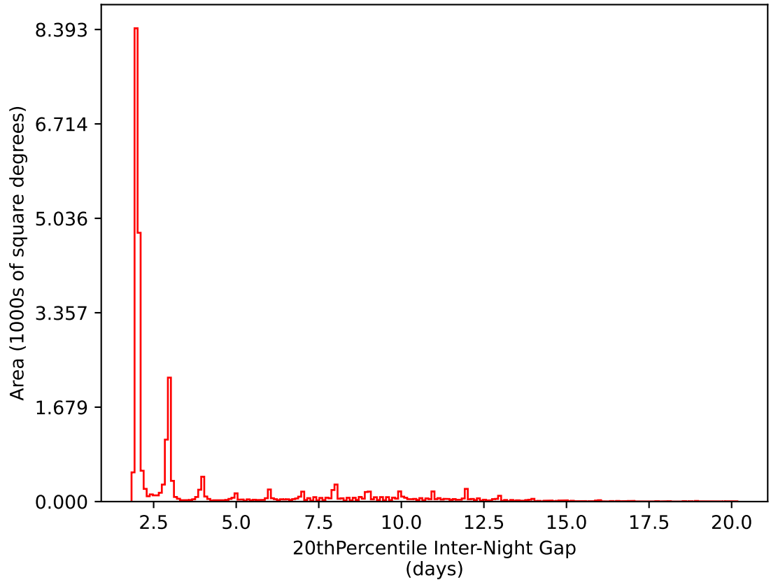
too_elab_r8_d2_giz_v3.4_10yrs All sky i band: 20thPercentile Inter-Night Gap
