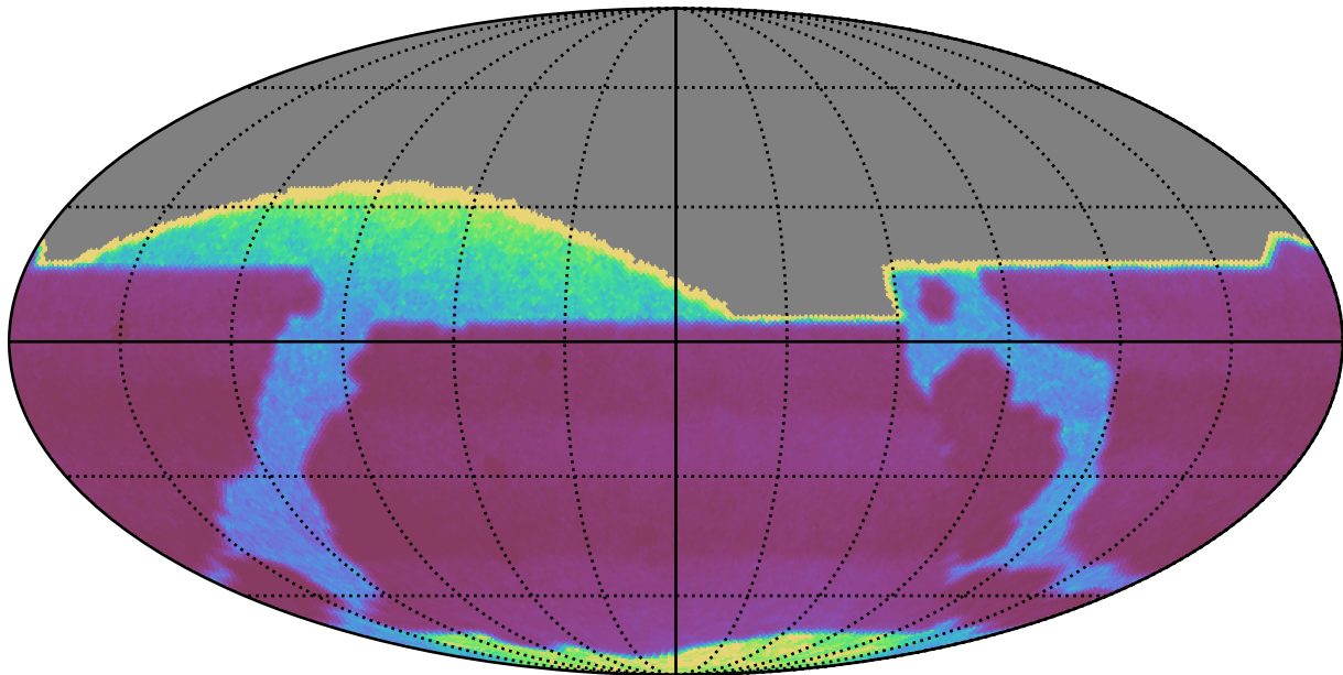
too_elab_r8_d2_giz_v3.4_10yrs : properMotion
