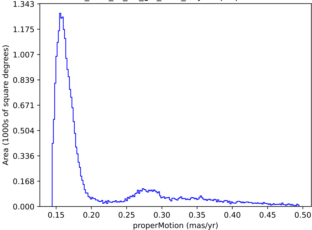
too_elab_r8_d2_giz_v3.4_10yrs : properMotion
