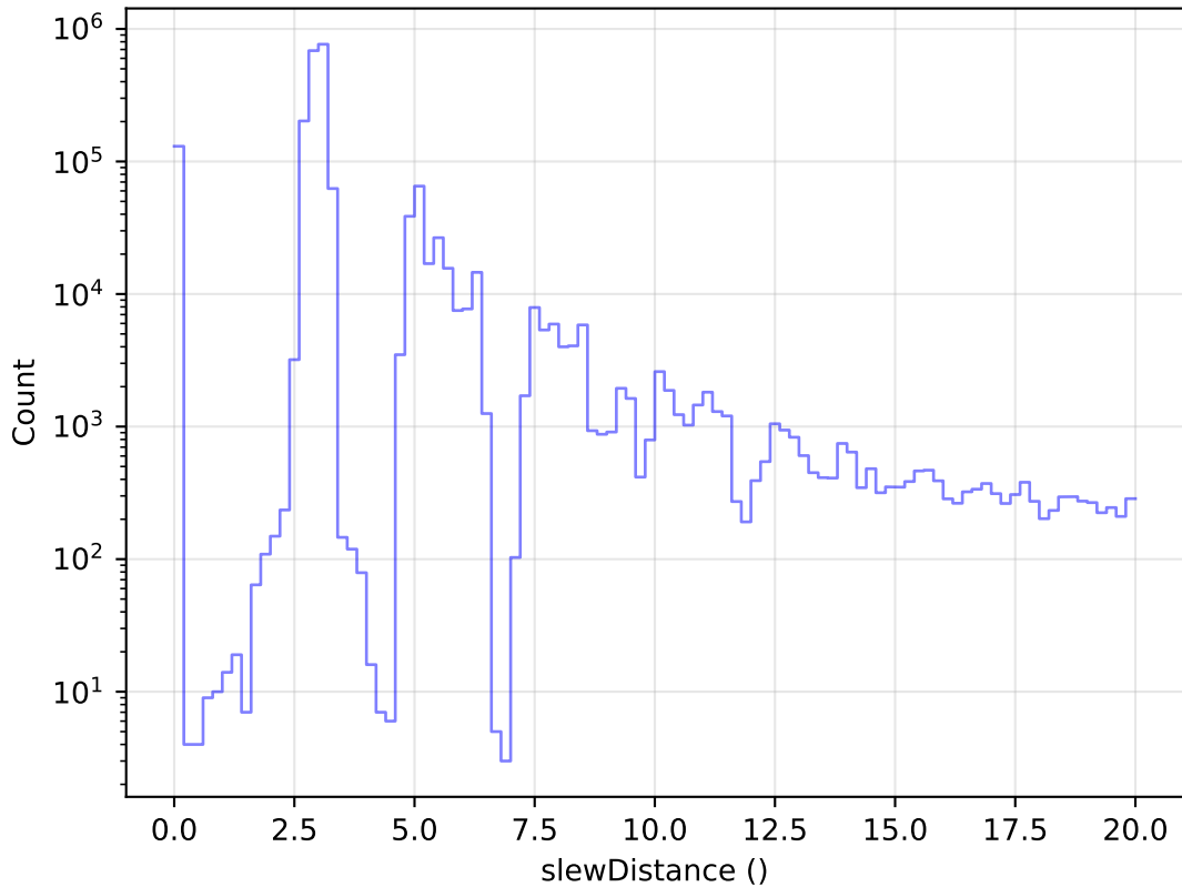
too_elab_r8_d2_giz_v3.4_10yrs All visits: Zoom Slew Distance Histogram
