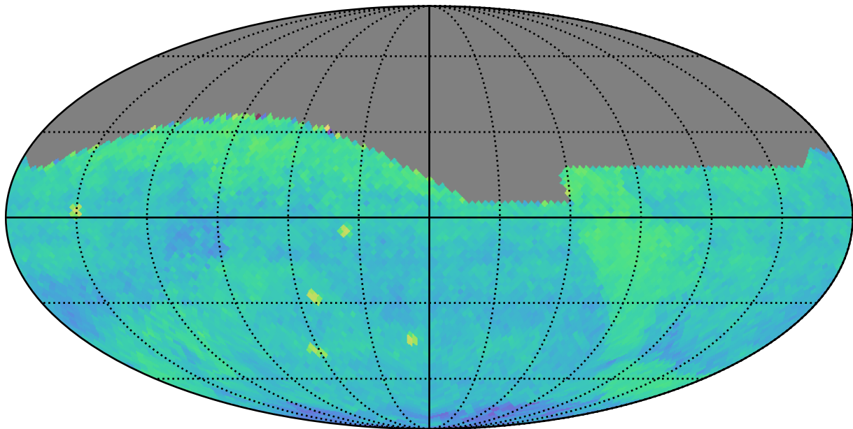
too_elab_r8_d2_giz_v3.4_10yrs (g or r or i): PairFraction
