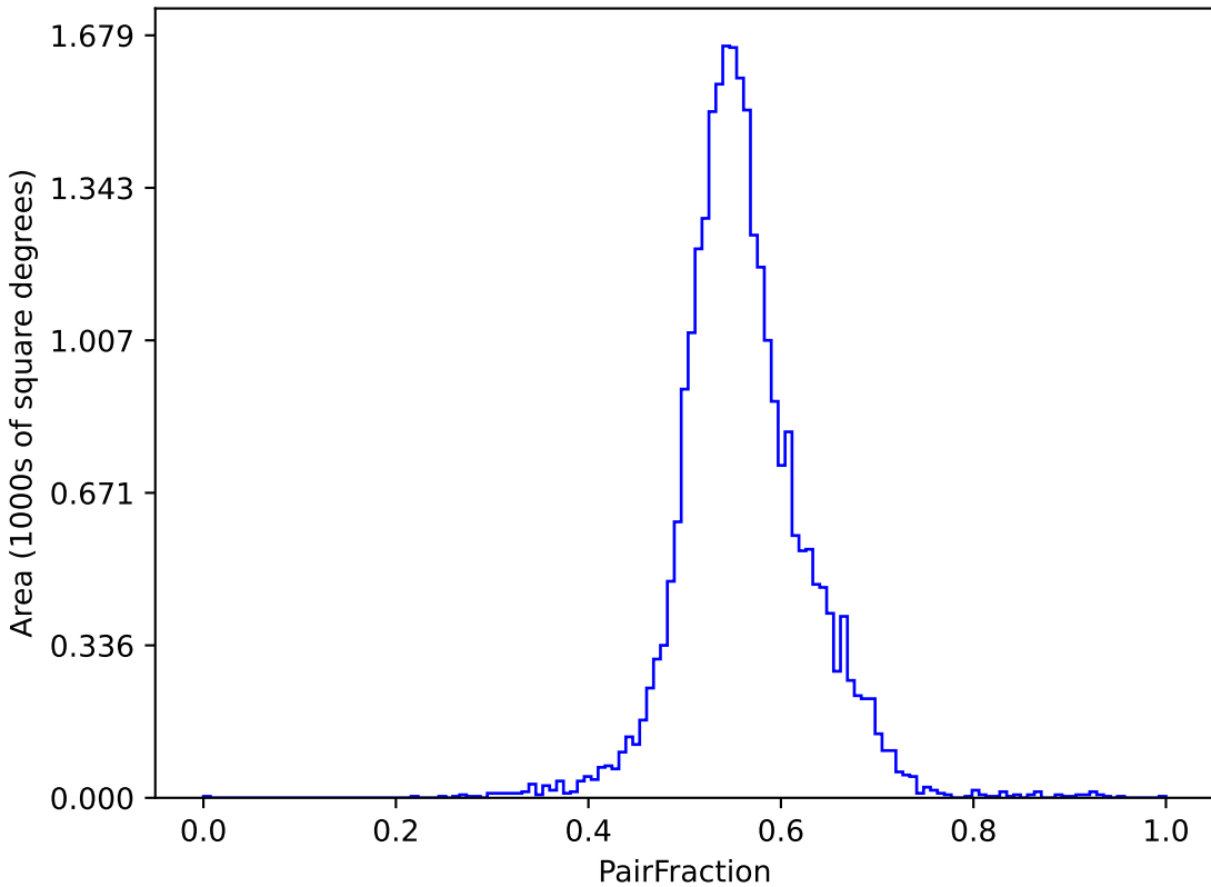
too_elab_r8_d2_giz_v3.4_10yrs (g or r or i): PairFraction
