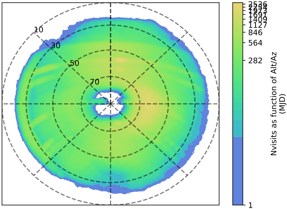
too_elab_r8_d2_giz_v3.4_10yrs r: Nvisits as function of Alt/Az
