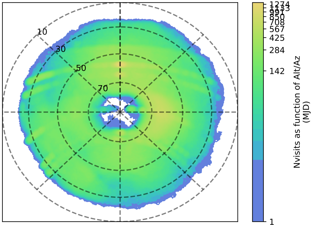
too_elab_r8_d2_giz_v3.4_10yrs g: Nvisits as function of Alt/Az
