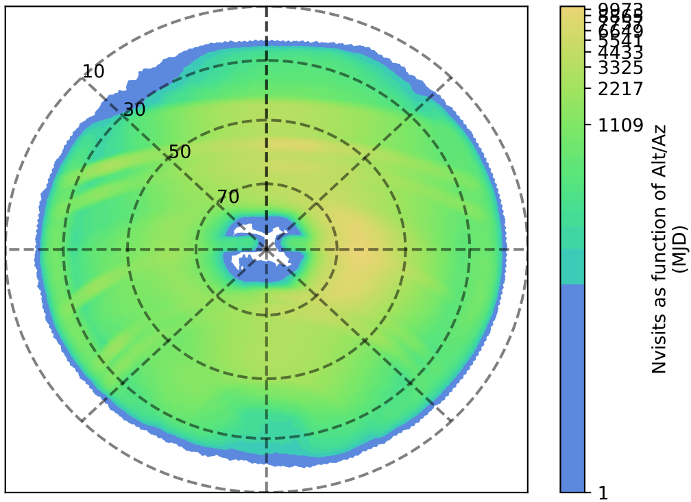
too_elab_r8_d2_giz_v3.4_10yrs : Nvisits as function of Alt/Az
