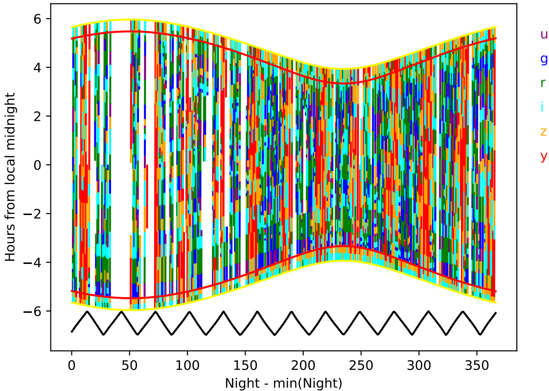
too_elab_r8_d2_giz_v3.4_10yrs year 8-9: Hourglass
