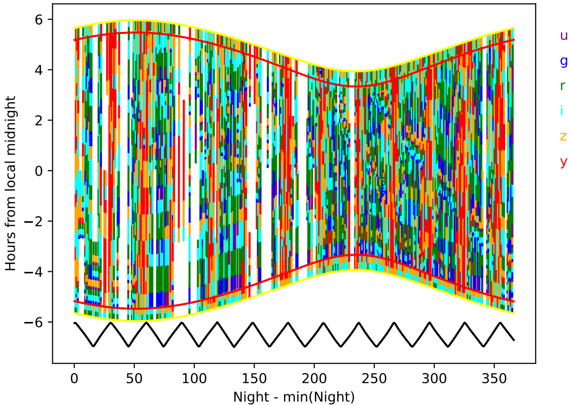
too_elab_r8_d2_giz_v3.4_10yrs year 1-2: Hourglass
