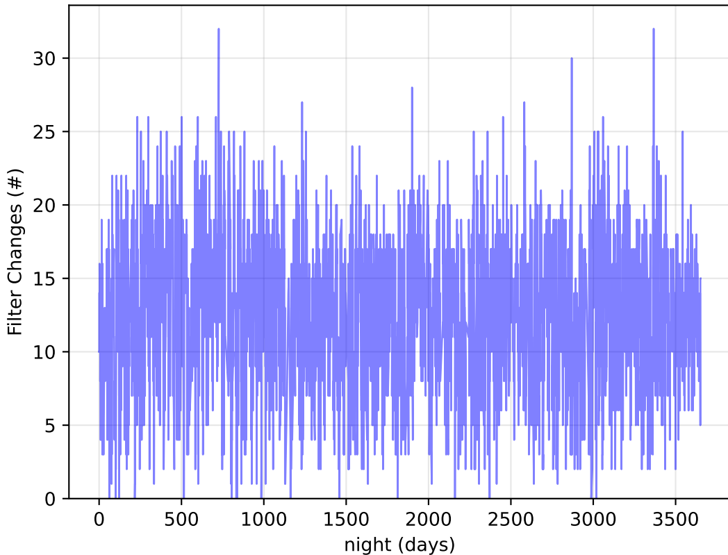
too_elab_r8_d2_giz_v3.4_10yrs : Filter Changes
