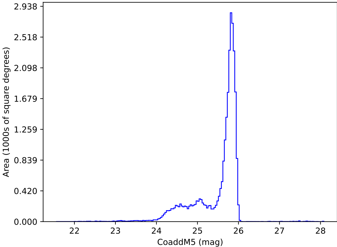
too_elab_r8_d2_giz_v3.4_10yrs z: CoaddM5
