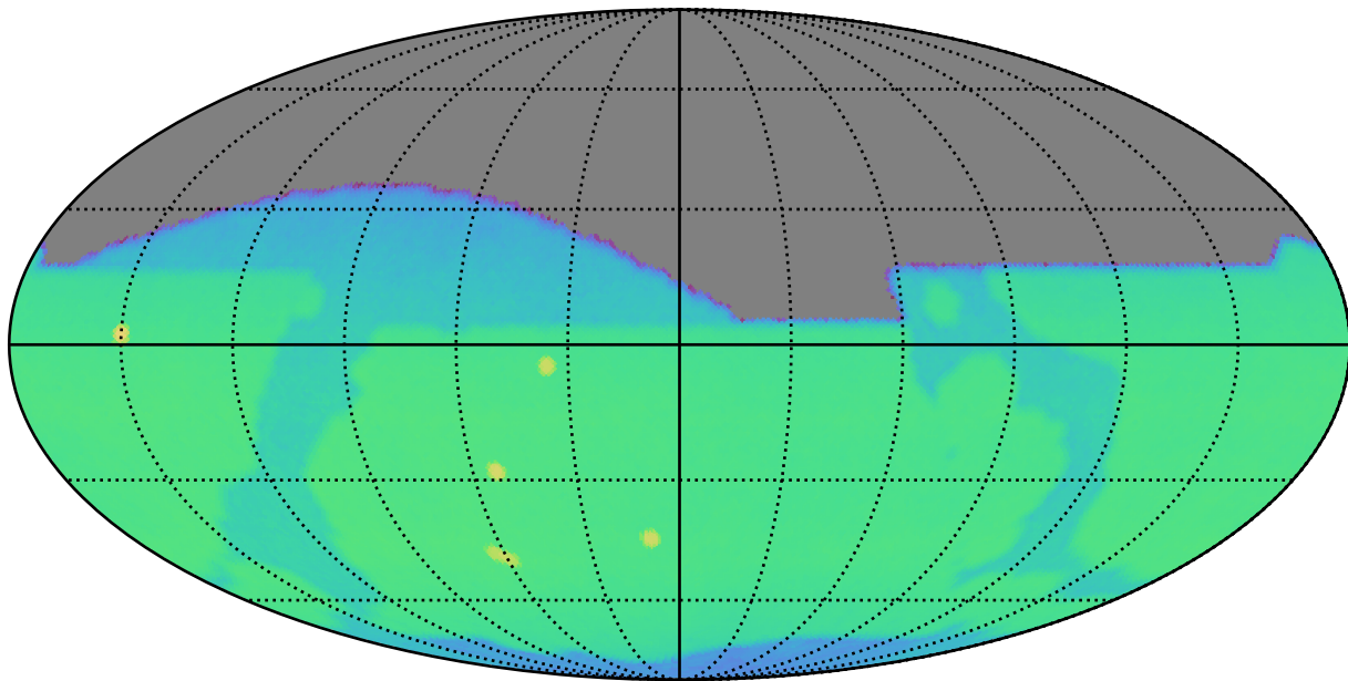
too_elab_r8_d2_giz_v3.4_10yrs i: CoaddM5
