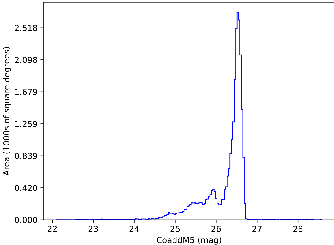
too_elab_r8_d2_giz_v3.4_10yrs i: CoaddM5
