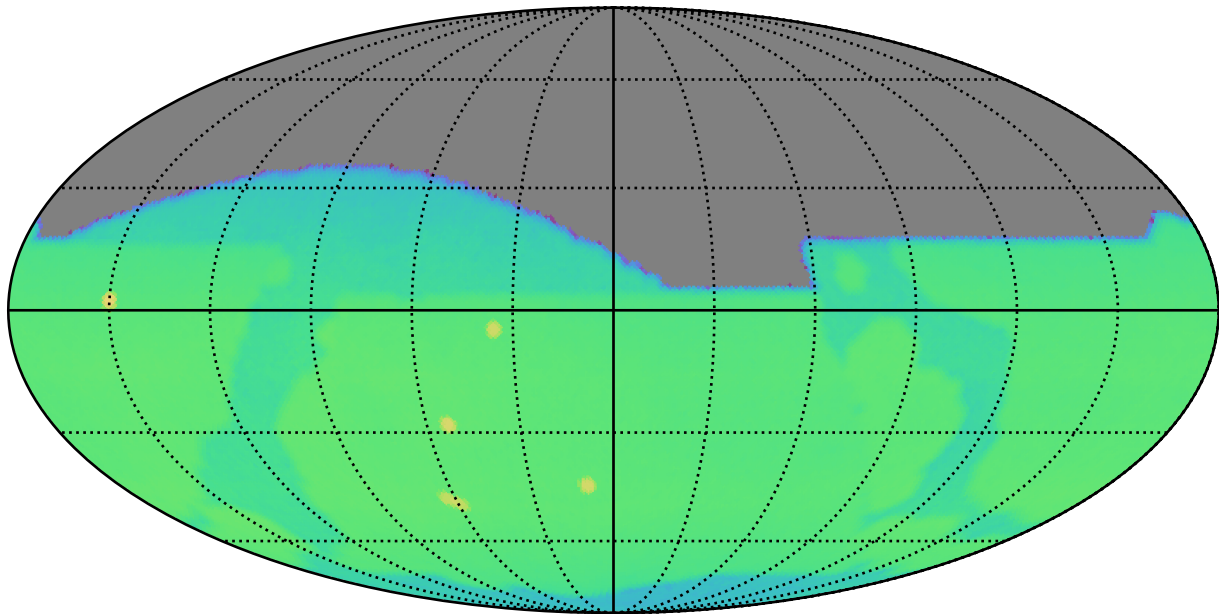
too_elab_r8_d2_giz_v3.4_10yrs : CoaddM5
